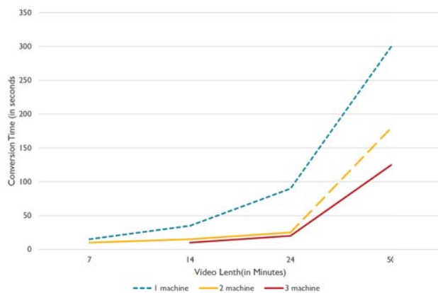
Fig. 7 VideoUpdateJob Performance
