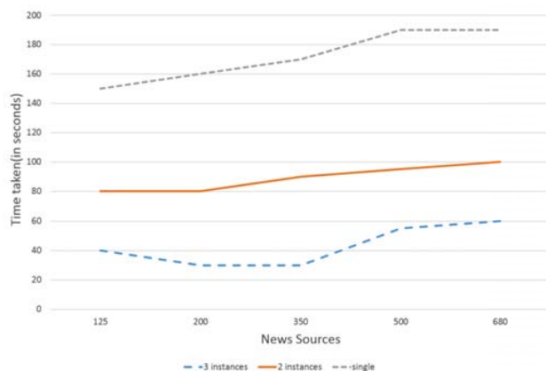
Fig. 3 NewsUpdateJob Performance
