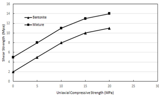
Fig. 3 Uniaxial compressive strength versus shear strength
