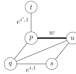
(a) e_{u,t} may be present
