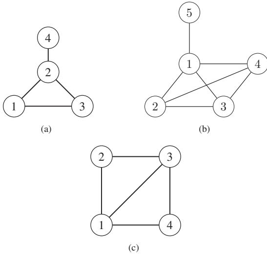
Fig. 1 Maximal subgraphs not present in the restricted interval graphs under consideration
