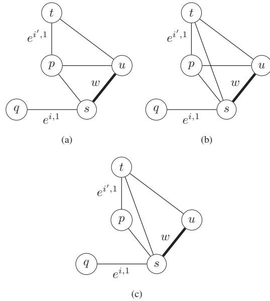
Fig. 3 Partial Sub-graph ( e_{p,q} and e_{q,u} may be present) induced by j_i, k_i, j_{i'}, k_{i'}, j_w, k_w (not all unique) in Case 3
