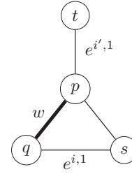
Fig. 2 Sub-graph induced by j_i, k_i, j_{i'}, k_{i'} in Case 1
