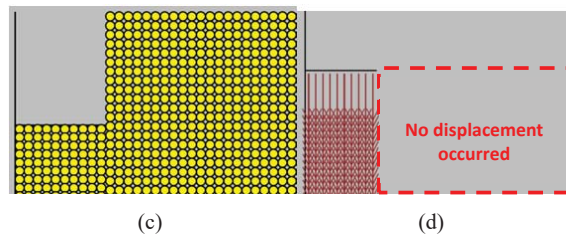
Fig. 6 Punching shear failure (contact bond=0, \phi=35^\circ , loose) (a) Model under uniform loading, (b) Displacement vectors of punching shear failure (c) Close-up view for punching shear failure and (d) Close-up view of punching shear failure
