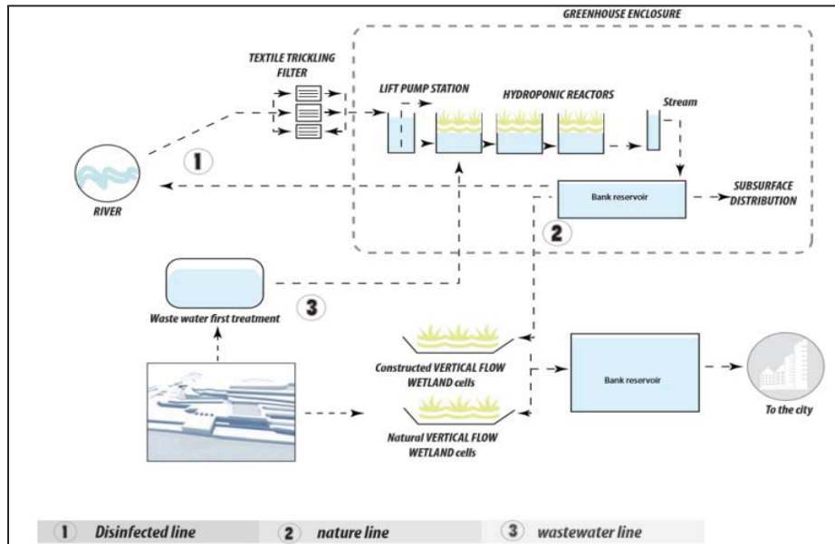
Fig. 11 The system application at the building level
