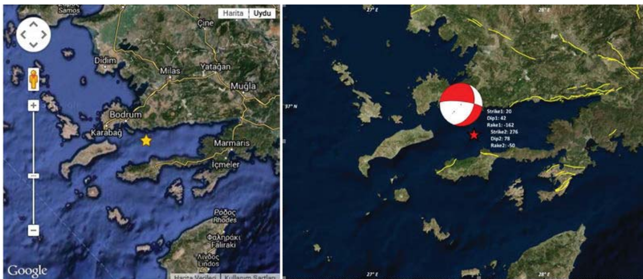
Fig. 5 On May 29th, 2015 at 11:02, an earthquake occurred in the Gökova Bay and its Focal mechanism solution [19]
