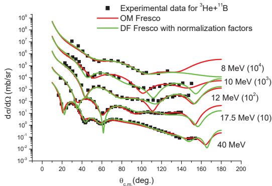
Fig. 4 Angular distributions for ^3\text{He}+^{11}\text{B} elastic scattering at ^3\text{He} energies (8, 10, 12, 17.5, 40 MeV) where (red line) represents the optical model calculations, (green line) represents the double folding calculations and (dots) represents the experimental data.
