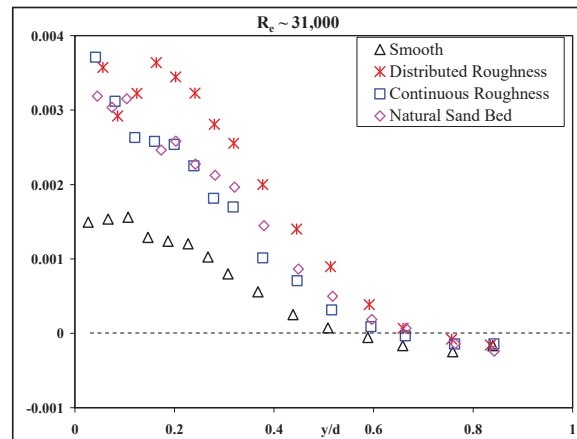
Fig. 4 Reynolds shear stress distribution for flow over different bed conditions
