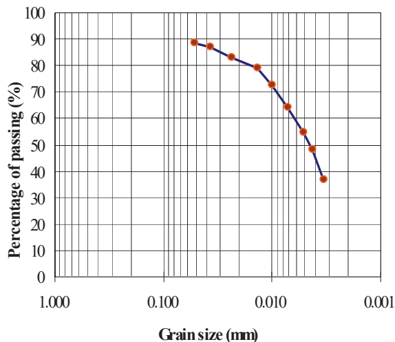
Fig. 2 Particle size distribution of dredged fill
