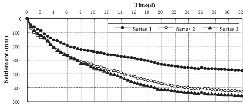
Fig. 9 Curves of settlement with time
