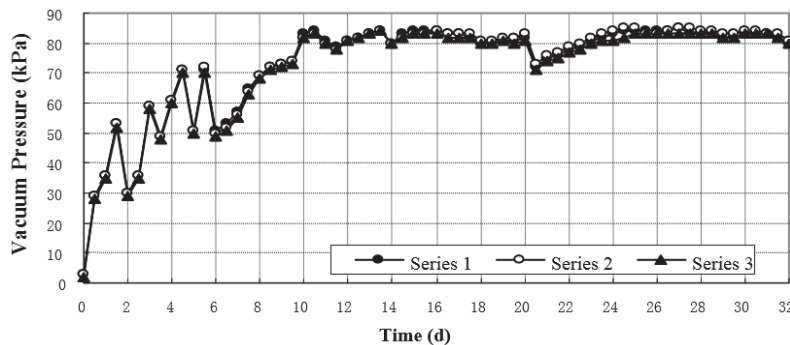
Fig. 8 Curves of vacuum pressure under the membrane
