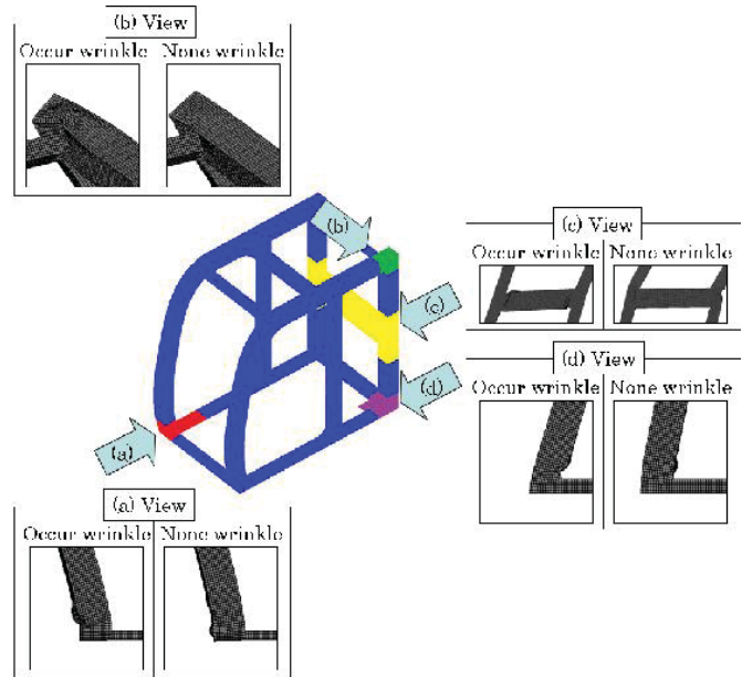
Fig. 3 Deformation View
