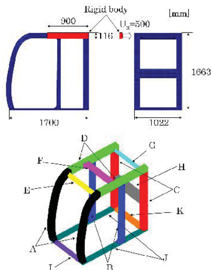
Fig. 1 Analysis model
