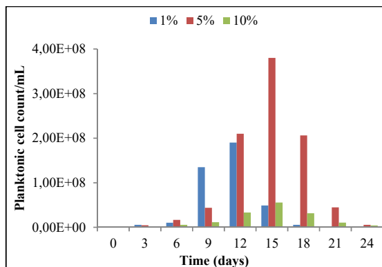
Fig. 5 Change in planktonic cell count with time
