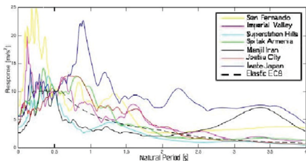
Fig. 7 Response spectrum of selected ground motions
