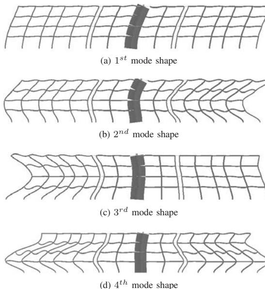
Fig. 4 First four natural mode shapes of the model according to SeismoStruct
