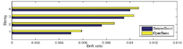
Fig. 6 Interstorey drifts from the nonlinear static analysis
