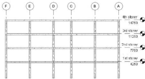
(b) Vertical projection of the structure
