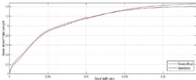
Fig. 11 Normalized base shear-control displacement relationship. The fracture strain of reinforcement steel in SeismoStruct is set equal to unity
