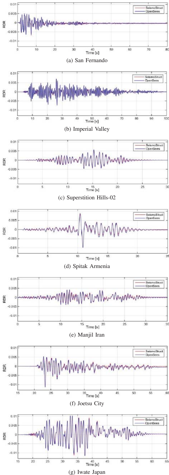
Fig. 8 RDR response history
