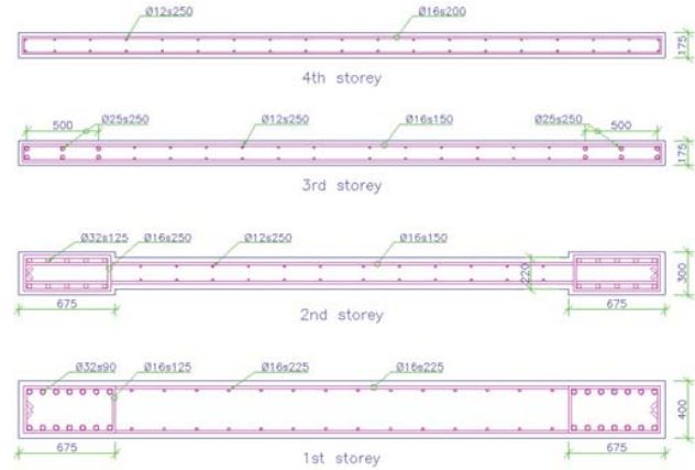
Fig. 2 Wall sections
