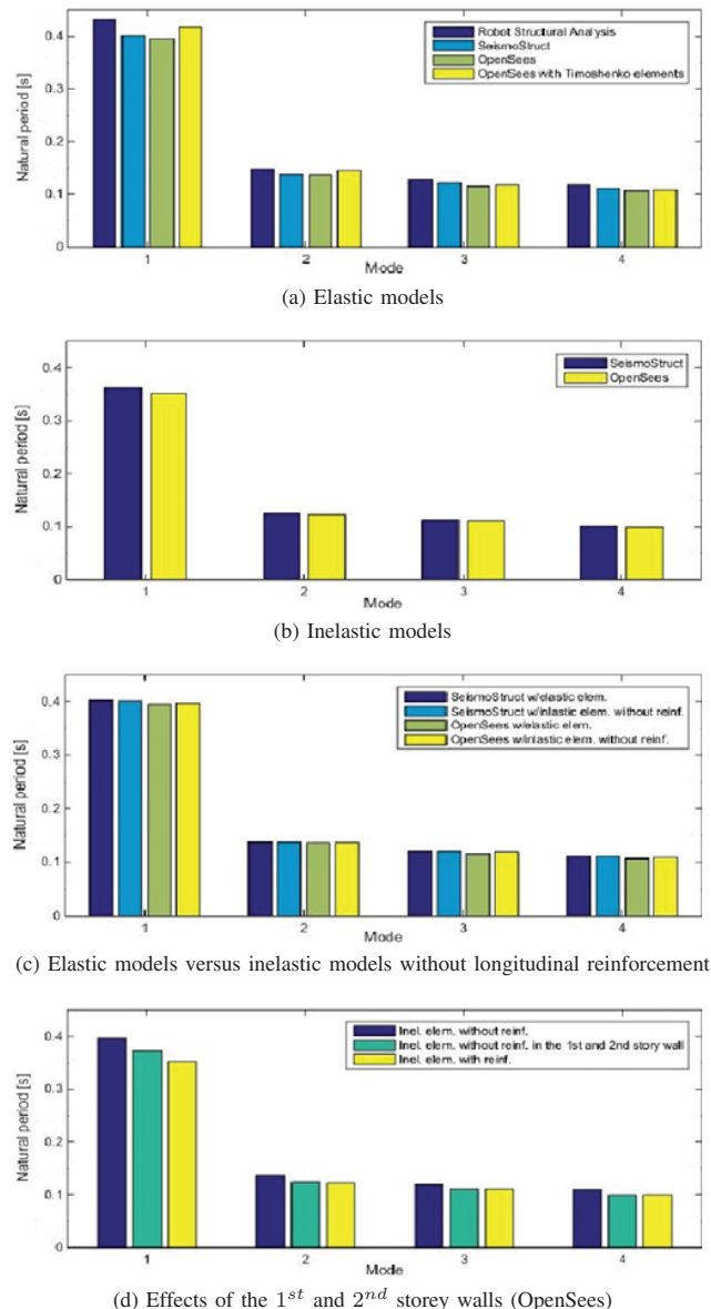
Fig. 3 Natural periods of the FEM-models
