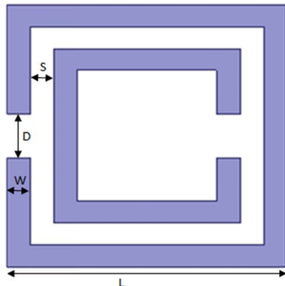
Fig. 1 The geometry configuration of a square SRR
