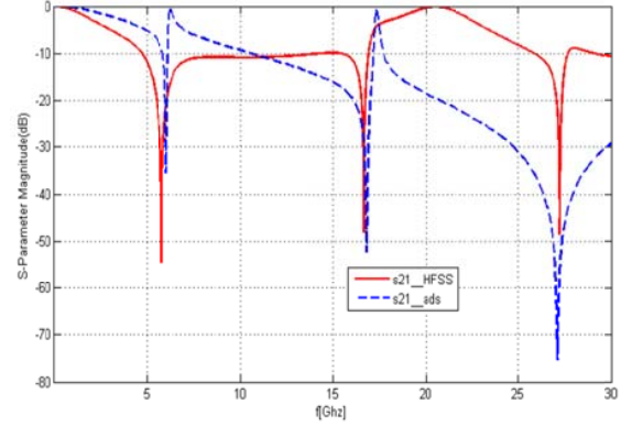
Fig. 7 The transmission coefficients of the SRR
