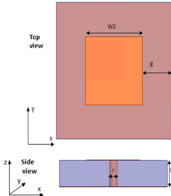
Fig. 3 The geometry configuration of HIS
