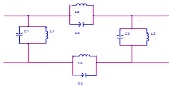
Fig. 2 The equivalent circuit model of SRR
