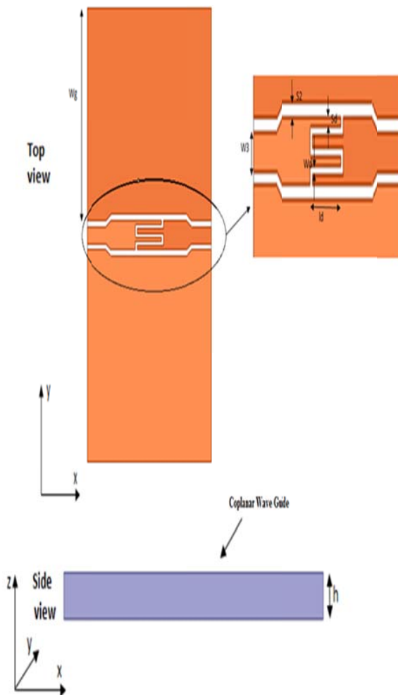
Fig. 5 The geometry configuration of IDC
