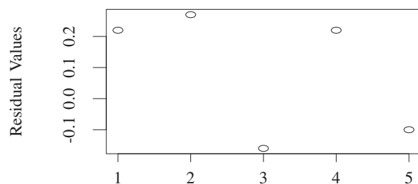
Fig. 7 Average by risk sources Our Model vs Estimation
