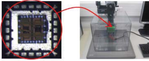
Fig. 11 QFN cavity with a Thermal Test Chip (TTC-1002) and PCB test board in a controlled environment-still air (enclosure)
