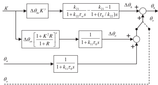
Fig. 2 Block diagram representation of the differential equations
