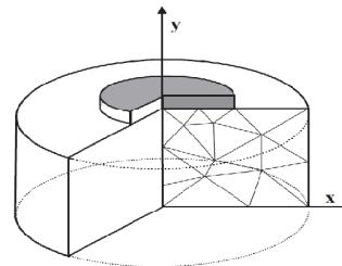
Fig. 2 Axisymmetric problem, [25]
