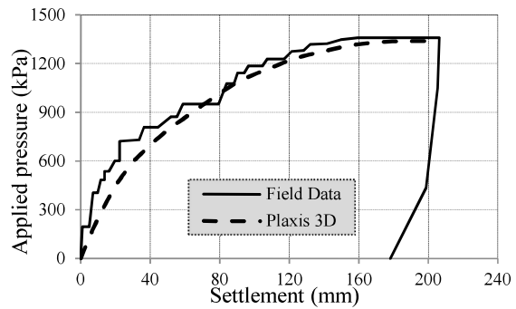
Fig. 4 Comparison of Plaxis 2D AE modeling results with real load-displacement behaviour for a field footing done by [15]
