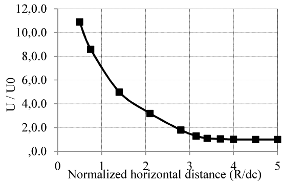
Fig. 7 Variation of excess pore pressure within the clay with distance from the column axis (displacement degree = 0.2 m)
