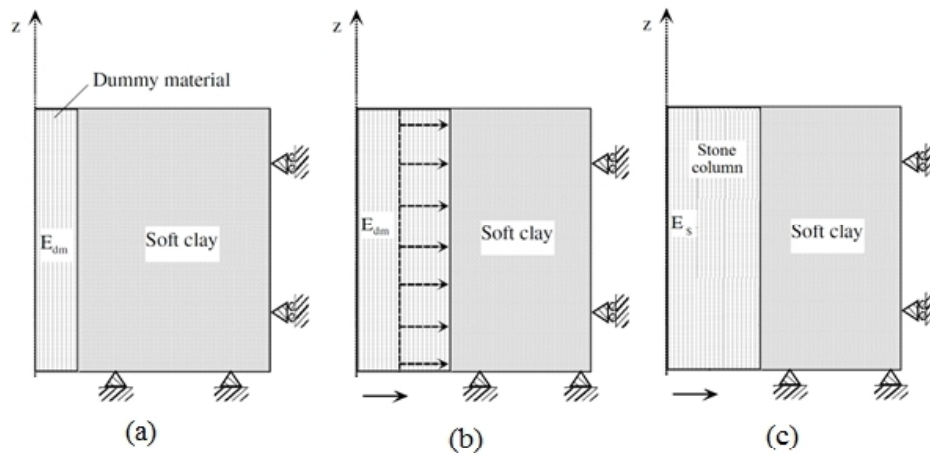
Fig. 5 Principle of stone column expansion using the dummy material
