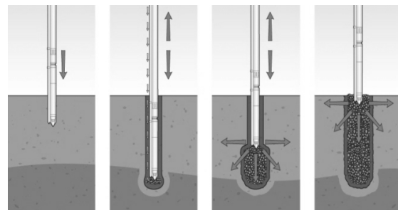
Fig. 1 Vibro displacement by dry bottom-feeding method, [16]
