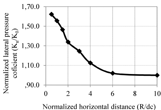
Fig. 8 Variation of stress within the clay with distance from the column axis (displacement degree = 0.2 m)
