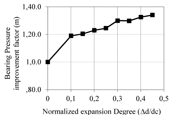
Fig. 10 Effect of expansion degree of the installed stone column on bearing capacity of reinforced footing
