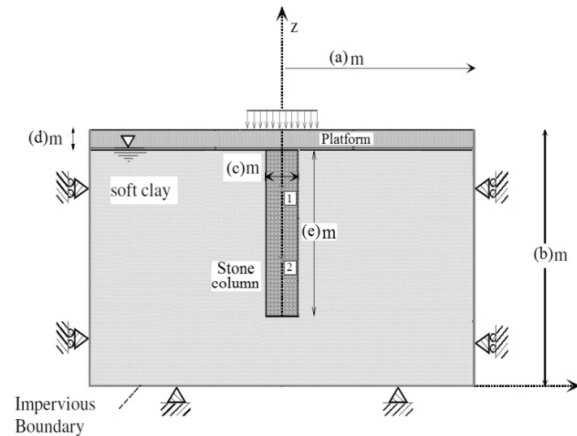
Fig. 3 Boundary conditions in studied model
