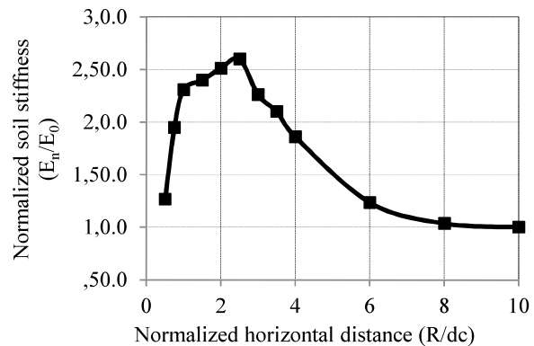
Fig. 9 Variation of stiffness of clay with distance from the column axis (displacement degree = 0.2 m)
