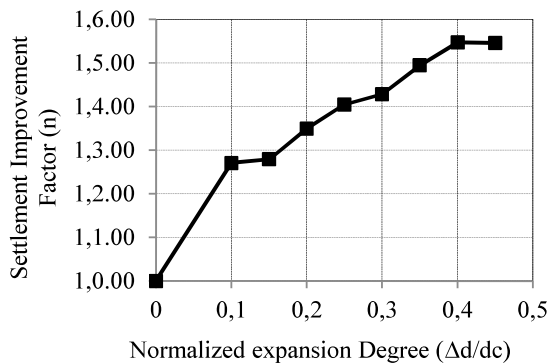
Fig. 11 Effect of expansion degree of the installed stone column on settlement of reinforced footing
