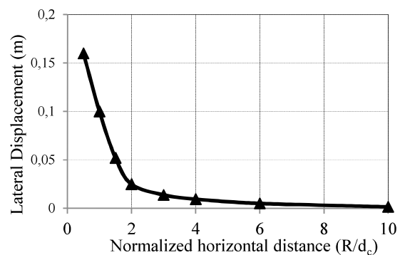
Fig. 6 Variation of lateral displacement within the clay with distance from the column axis (displacement degree = 0.2 m)
