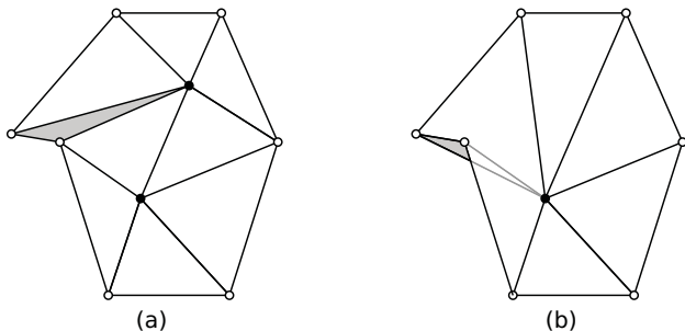
Fig. 1 Mesh foldover example: mesh before (a) and after (b) the collapse that caused a foldover
