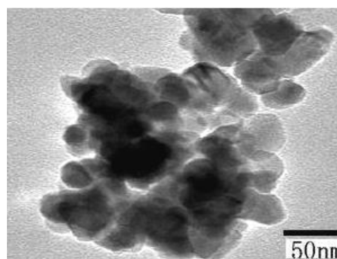
Fig. 3 TEM image of CdO nanoparticles
