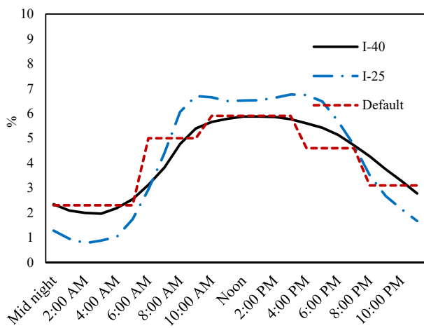
Fig. 5 Hourly Truck Distribution
