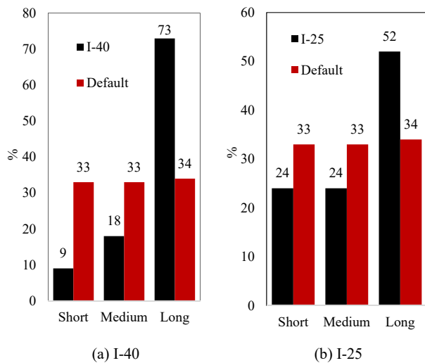
Fig. 9 Wheelbase Distribution
