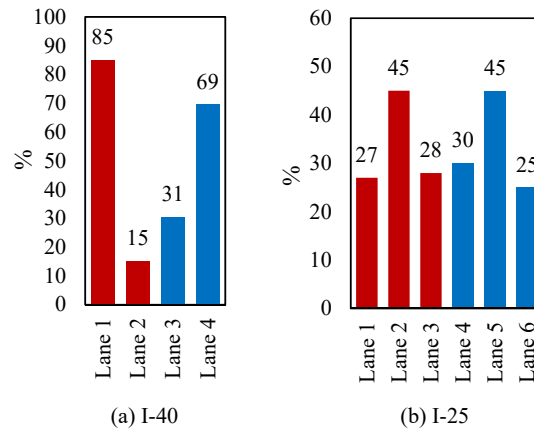
Fig. 3 Lane Distribution Vehicle Operational Speed
