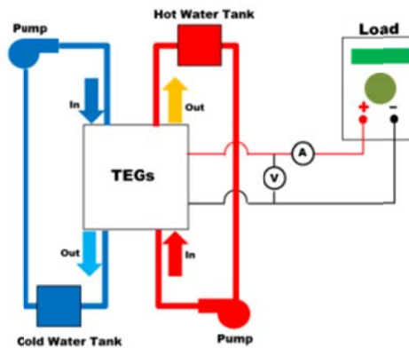
Fig. 8 System schematic
