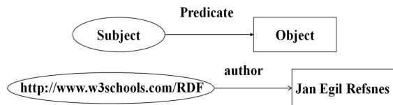
Fig. 1 RDF Data Model Graph
