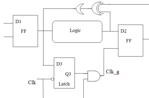
Fig. 3 Data driven clock gating
