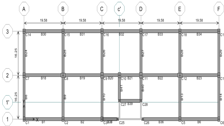
Fig. 2 Column-beam layout Plan (all dimensions are in feet)
