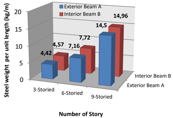
Fig. 7 Steel weights per unit length of beam in transverse direction
