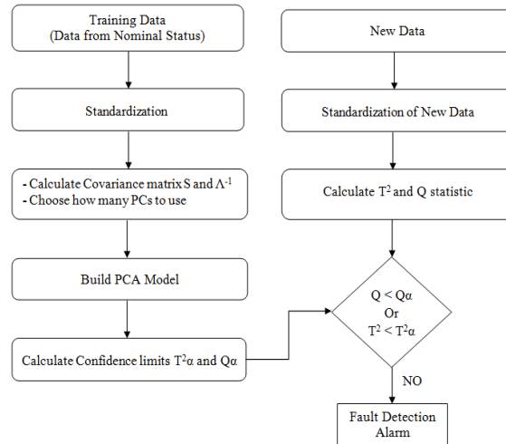
Fig. 2 PCA Fault detection algorithm framework
