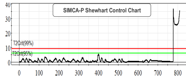
Fig. 14 SIMCA-P Shewhart control charts for process shifts
