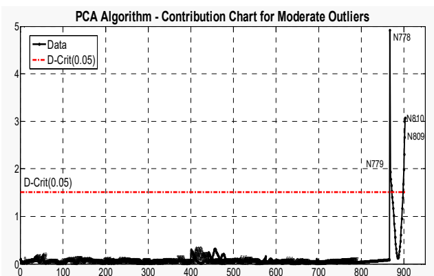
Fig. 10 PCA algorithm contribution plot
