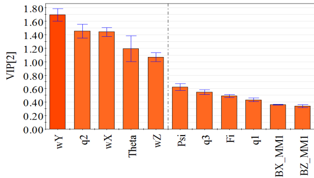
Fig. 8 SIMCA-P variables importance in projection
