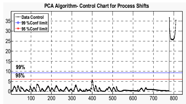
Fig. 13 PCA algorithm control charts for process shifts
