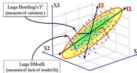
Fig. 3 Establishing score plot for three variables
