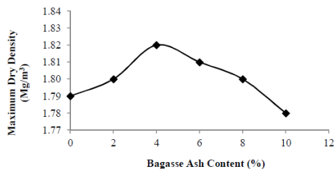
Fig. 14 Variation of MDD with bagasse ash treatment for soil-RAP mix [2]
