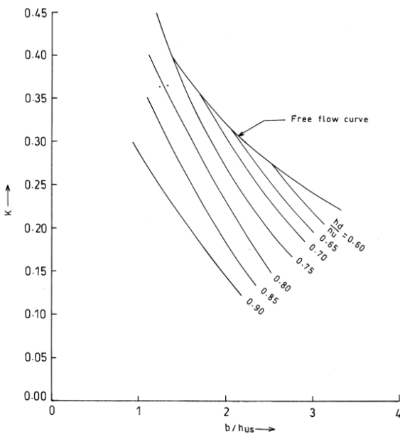
Fig. 5 Plotted curves for different submergence ratio for 1.5:1 flowmeter
