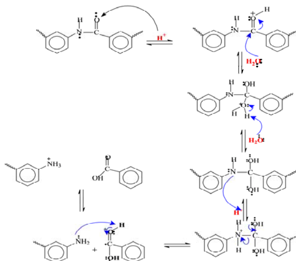
Fig. 6 Hydrolysis mechanism catalyzed by an acid of the amide bond in Nomex®
