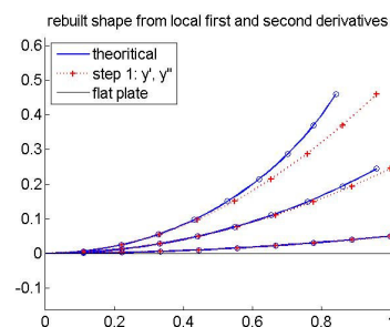
Fig. 4 y coordinates computed with a fifth order spline
