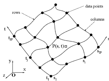
Fig. 1 Kriging interpolation of a 3D surface
