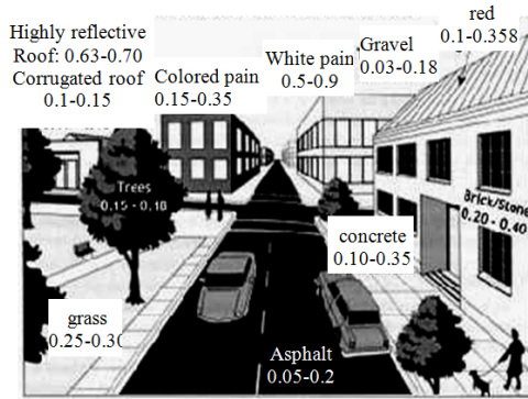
Fig. 4 Albedo values of an urban area
