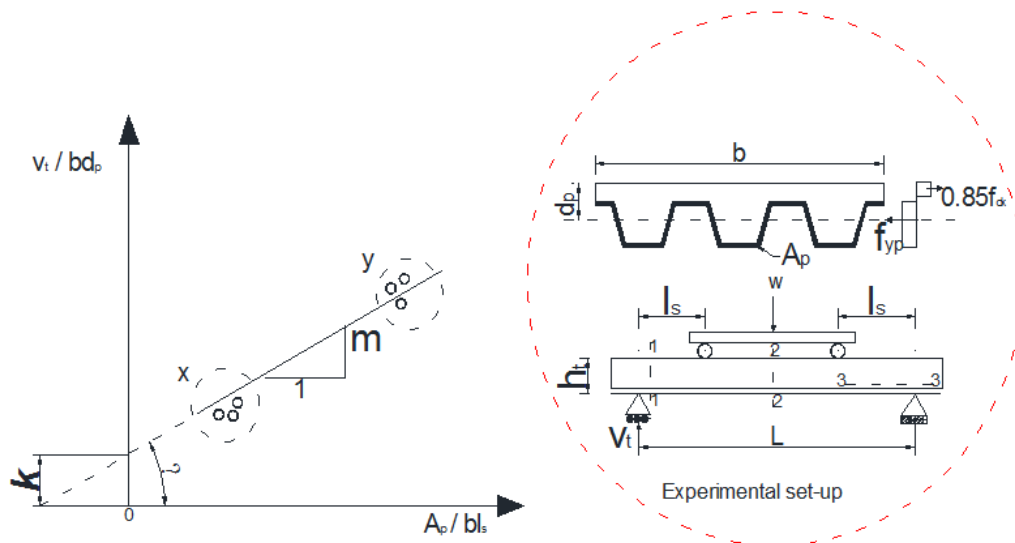
Fig. 1 Schematic m-k parameters determination from the plot of vertical shear against shear bond
