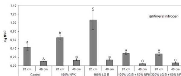
Fig. 3 N_{\min} loss (sum of nitrate and ammonium nitrogen) from topsoil (0 – 20 cm) and subsoil (20 – 40 cm); (mean values \pm SD, n = 3, different letters indicate significant differences)
