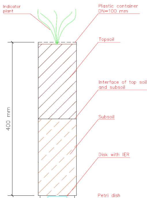
Fig. 1 Experimental container
