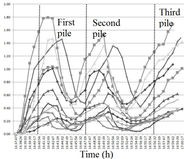
Fig. 7 Normalized responses of all sensors
