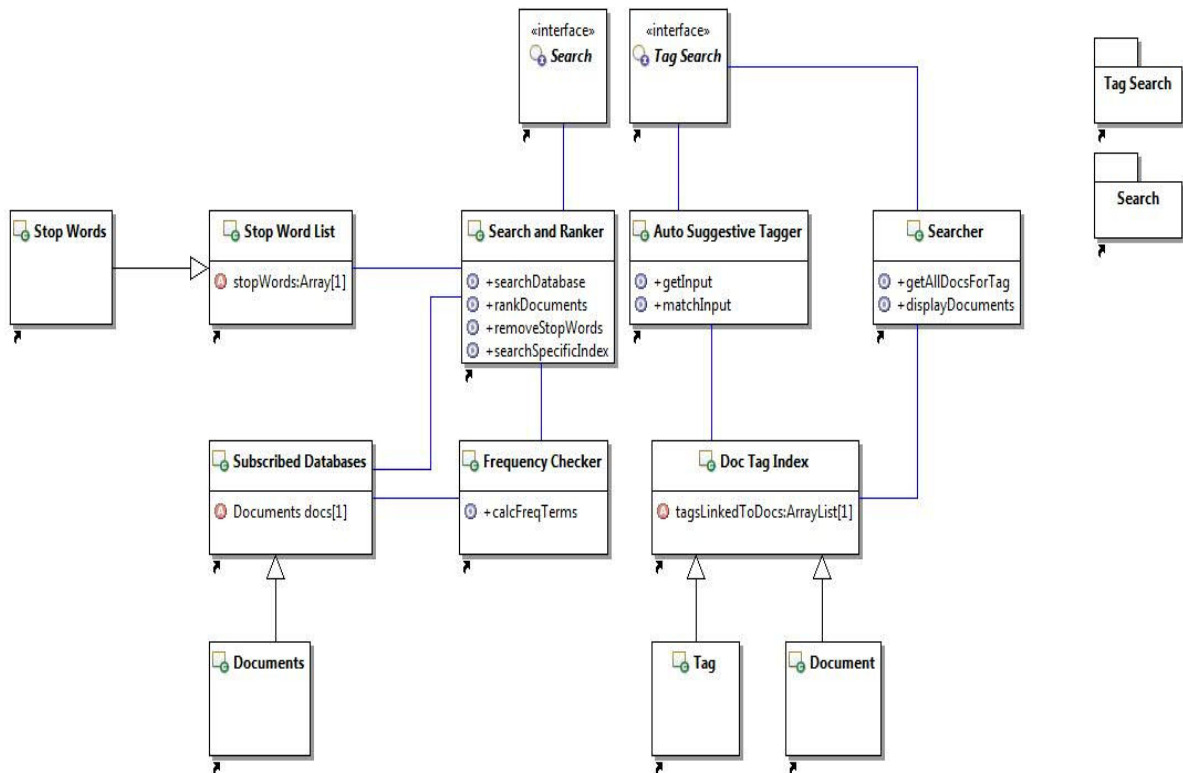
Fig. 10 The Class Diagram of RIS System
