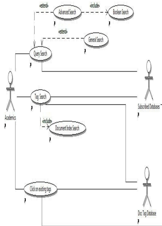
Fig. 7 The use case diagram of IRS
