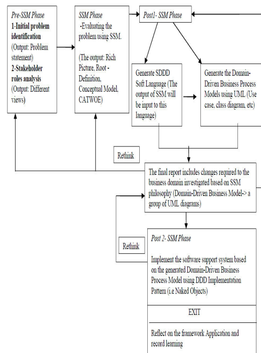
Fig. 2 The conception of SDDDF
