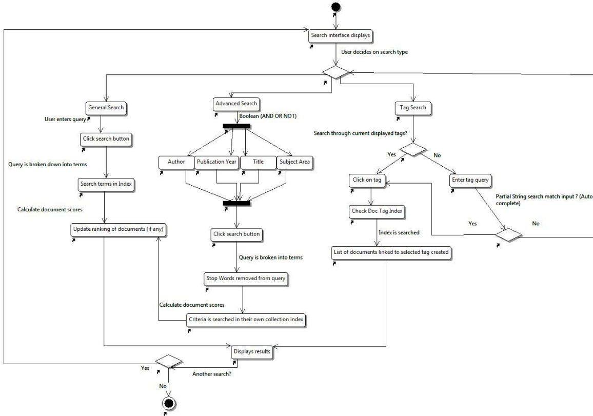
Fig. 9 Activity Diagram
