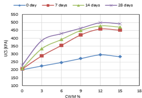
Fig. 11 Relationship between UCS and Percentages of CWM in Different Periods of Curing
