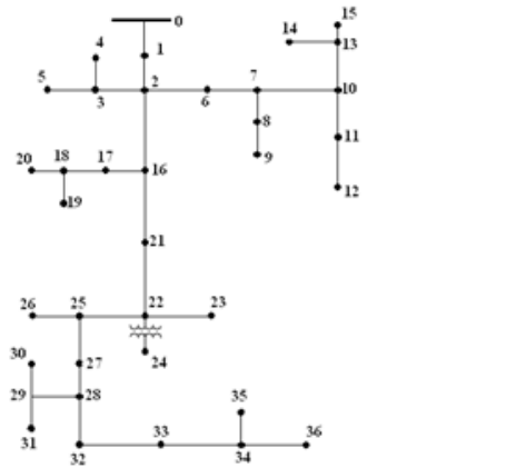
Fig. 3 Renumbered IEEE 37- node feeder
