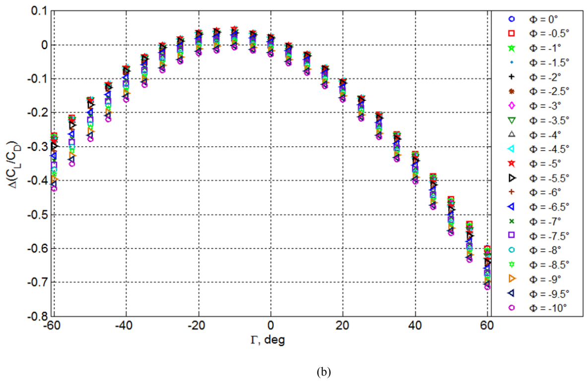
Fig. 4 Effects of Changing Winglet Cant and Twist angle on Aircraft Performance ( \Delta C_L/C_D ) at C_{L_0} \cong 0.6 : a) Wash-in (Positive Twist) and b) Wash-out (Negative Twist).
