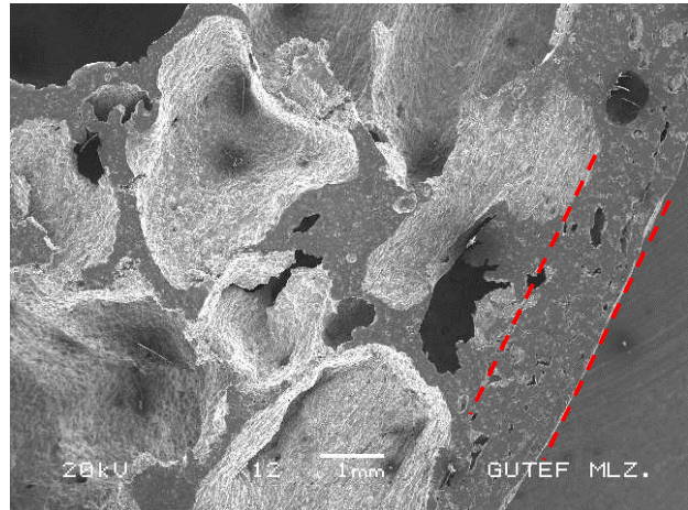
Fig. 6 Tensile region of bended specimen in 656°C
