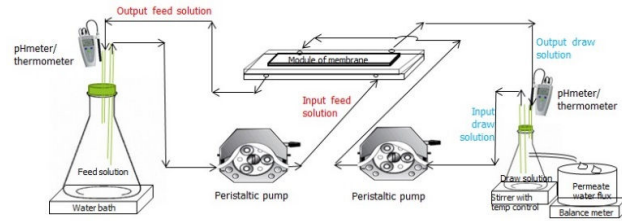
Fig. 1 Forward osmosis experimental apparatus
