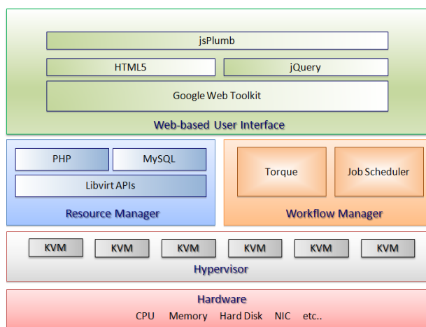
Fig. 2 Software architecture
