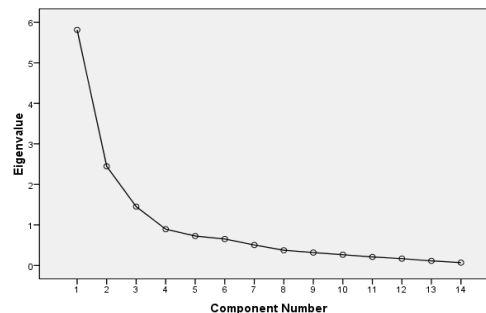
Fig. 1 Scree plot
