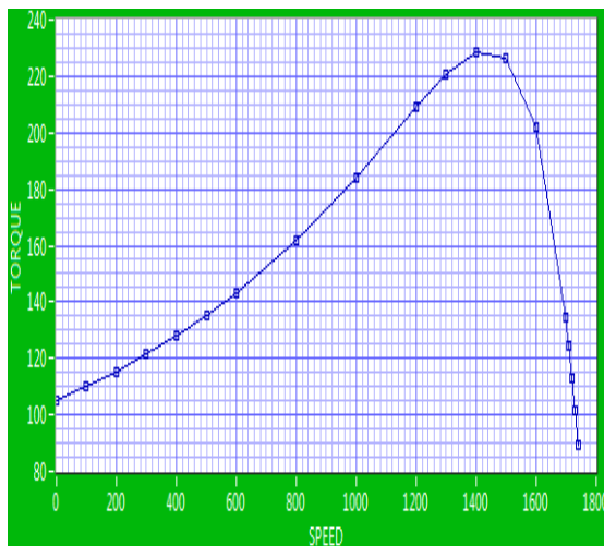
Fig. 4 Torque vs speed characteristics of induction motor
