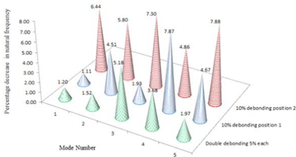
Fig. 6 Comparison of multiple debonding with equivalent area of single debonding
