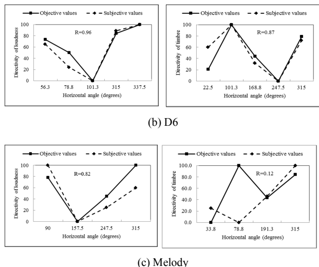
Fig. 4 Comparison between objective data and subjective data for particular tones and a melody. The left figures indicate the comparison results of directivity pattern of loudness, and the right figures indicate the comparison results of directivity pattern of timbre.
