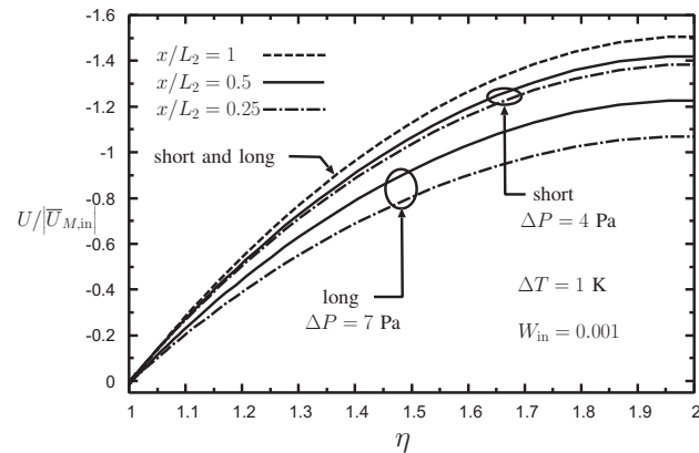
Fig. 3 Velocity profiles
