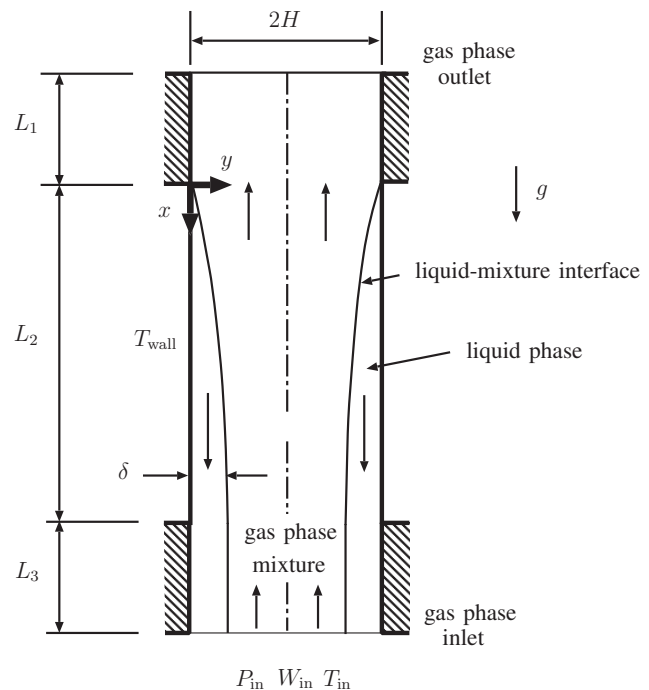
Fig. 1 Reflux condensation-model domain
