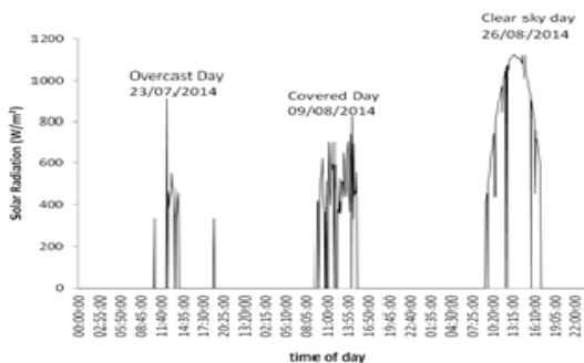
Fig. 2 Global solar radiation on the surface of the collector characteristic for three days
