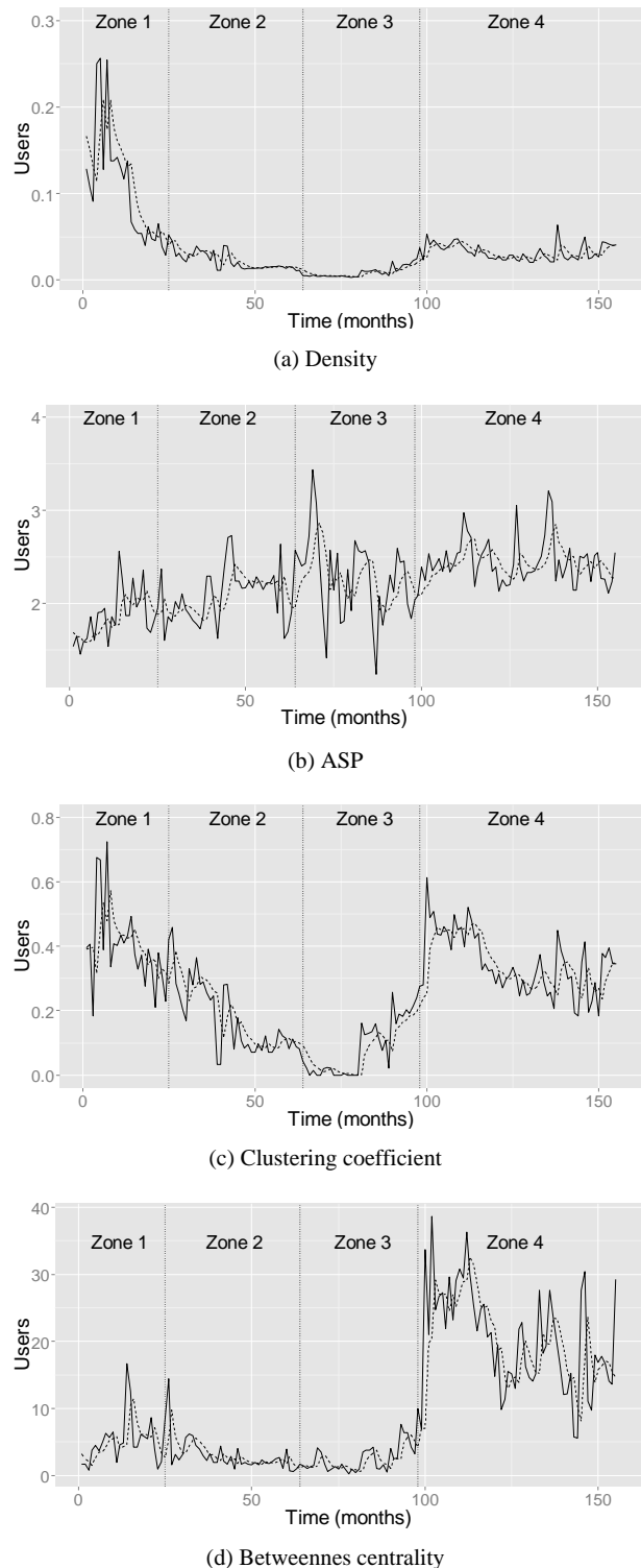
Fig. 3 Social network features evolution
