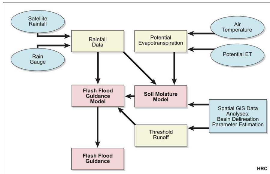
Fig. 1 Conceptual diagram of the CAFFG [5]
