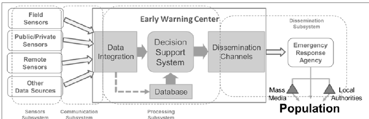
Fig. 3 Standard Early Warning System architecture
