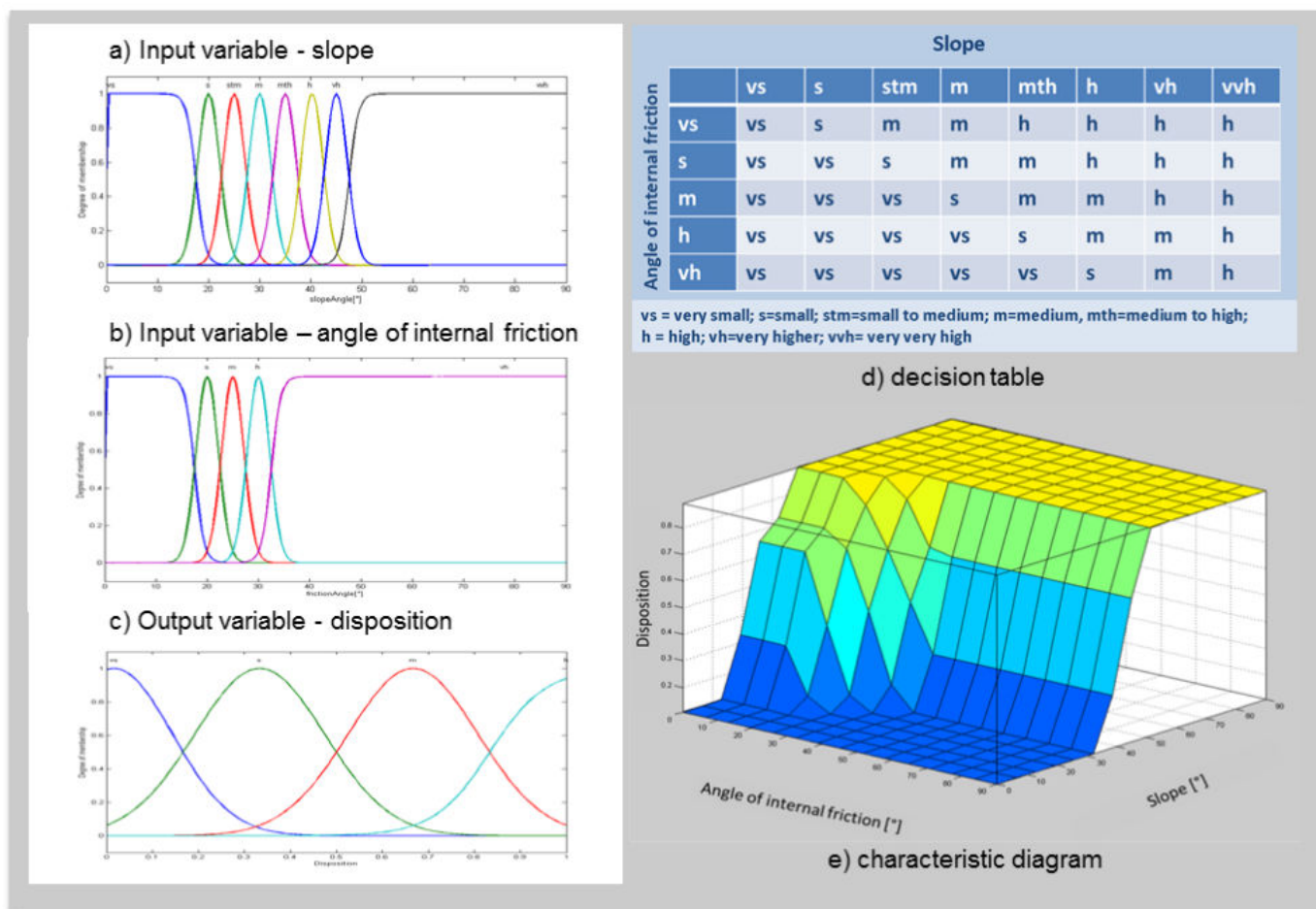
Fig. 5 Diagram of fuzzy expert systems from ELDEWAS [8]
