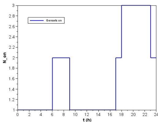
Fig. 3 Number of Diesel generators on
