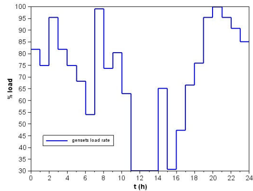
Fig. 4 Hourly load rate of each Diesel generator
