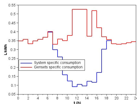
Fig. 6 Diesel and system specific consumptions
