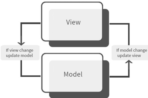
Fig. 1 Two-way data binding in Angular JS library
